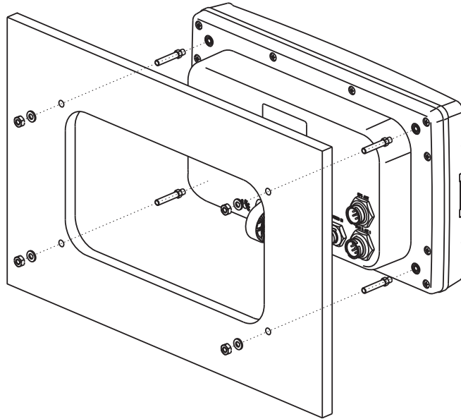
Figure 2.2a - Example of CP300 Flush installation
