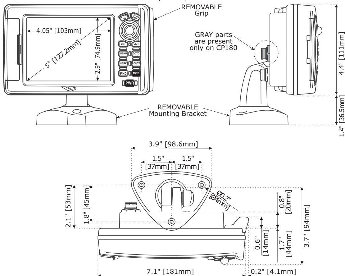
Figure 19.0 - CP180/CP180i Dimensions [inch/mm]
