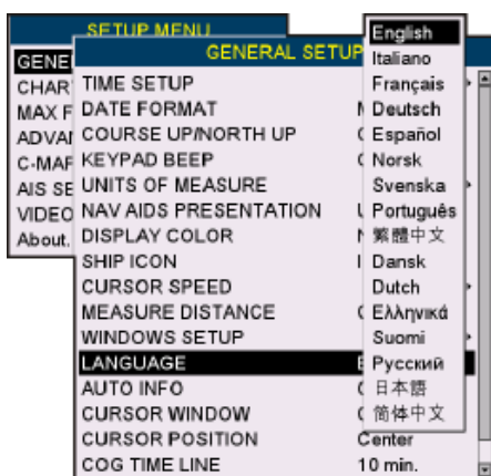
Figure 3.5 - Language Selection menu
