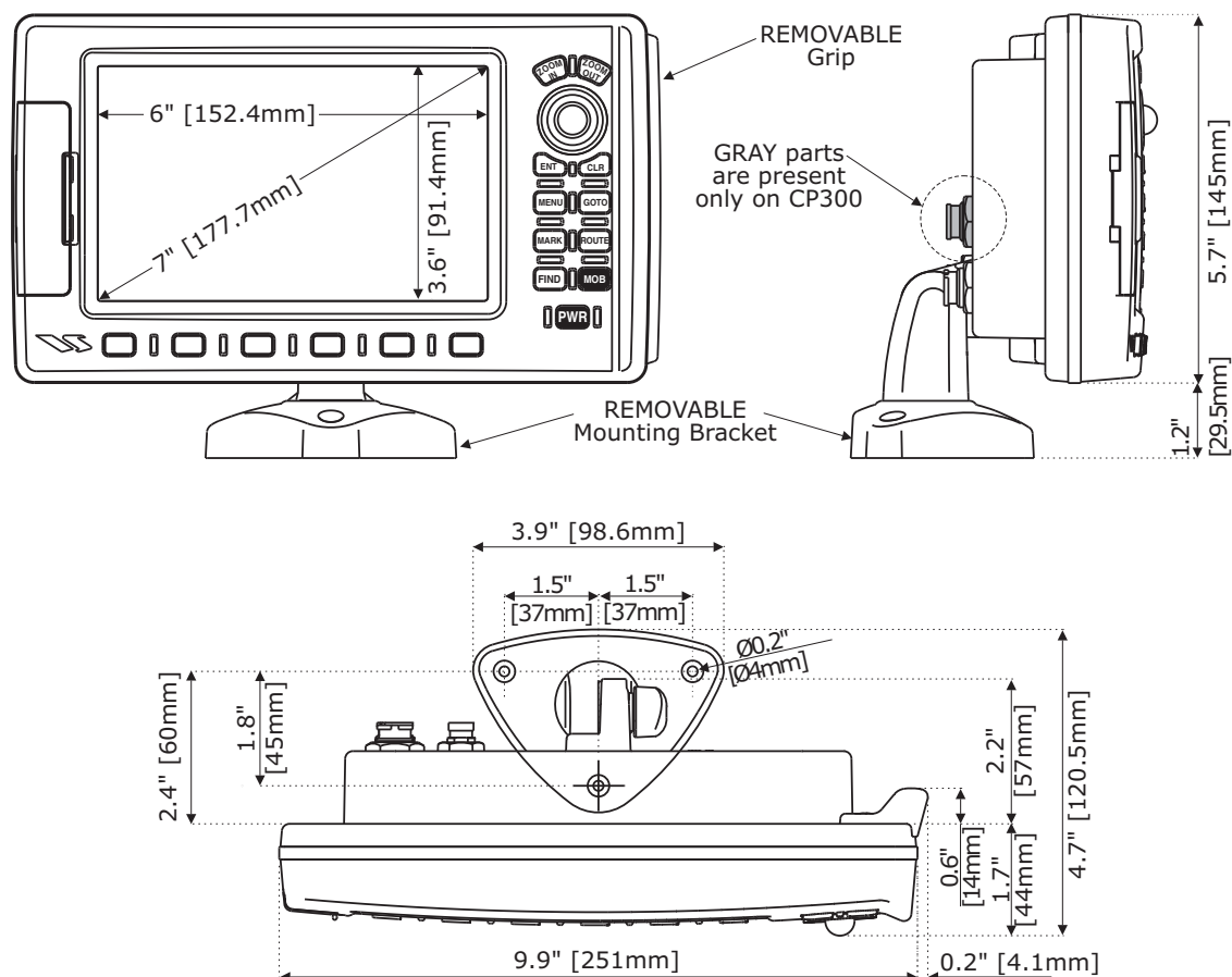
Figure 19.1 - CP300/CP300i Dimensions [inch/mm]
