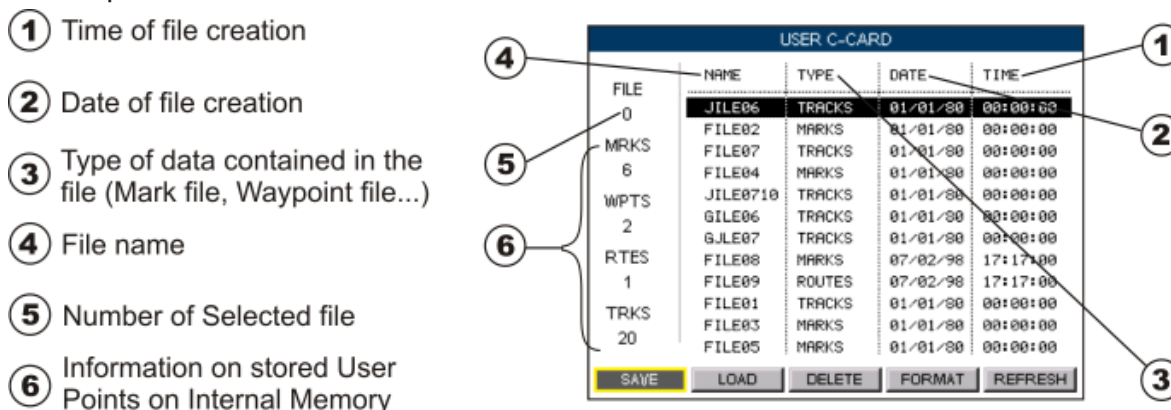
Figure 11.0 - User C-CARD Menu
