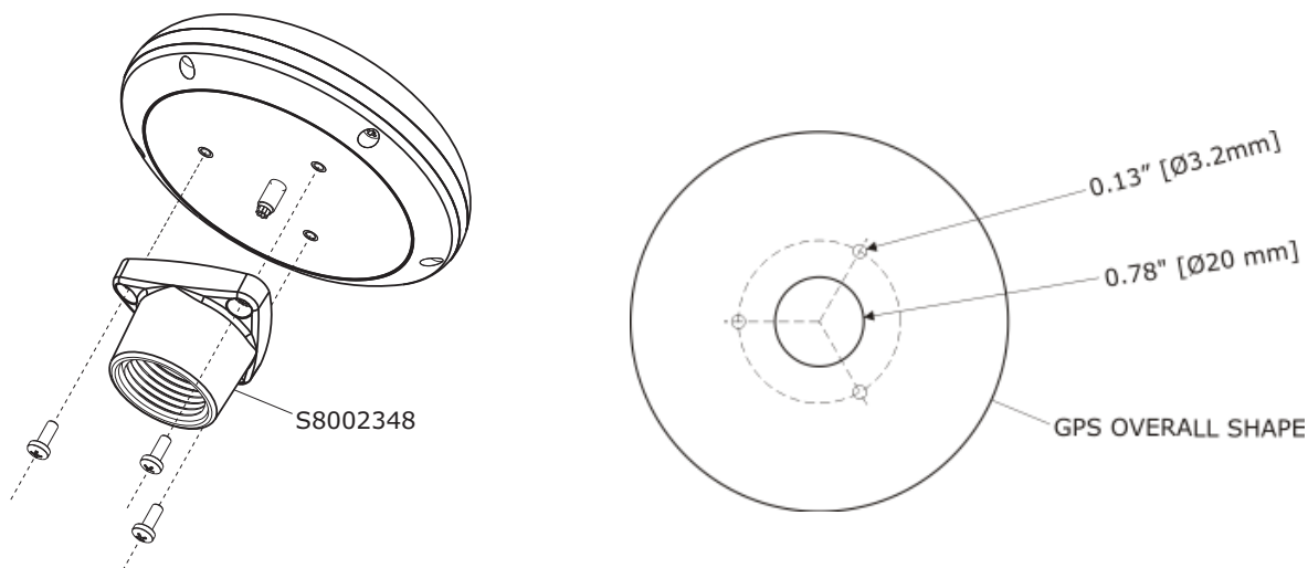
Figure 2.3.0 - Installing the External GPS Antenna
