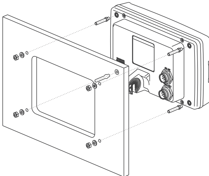
Figure 2.2 - Example of CP180 Flush installation
